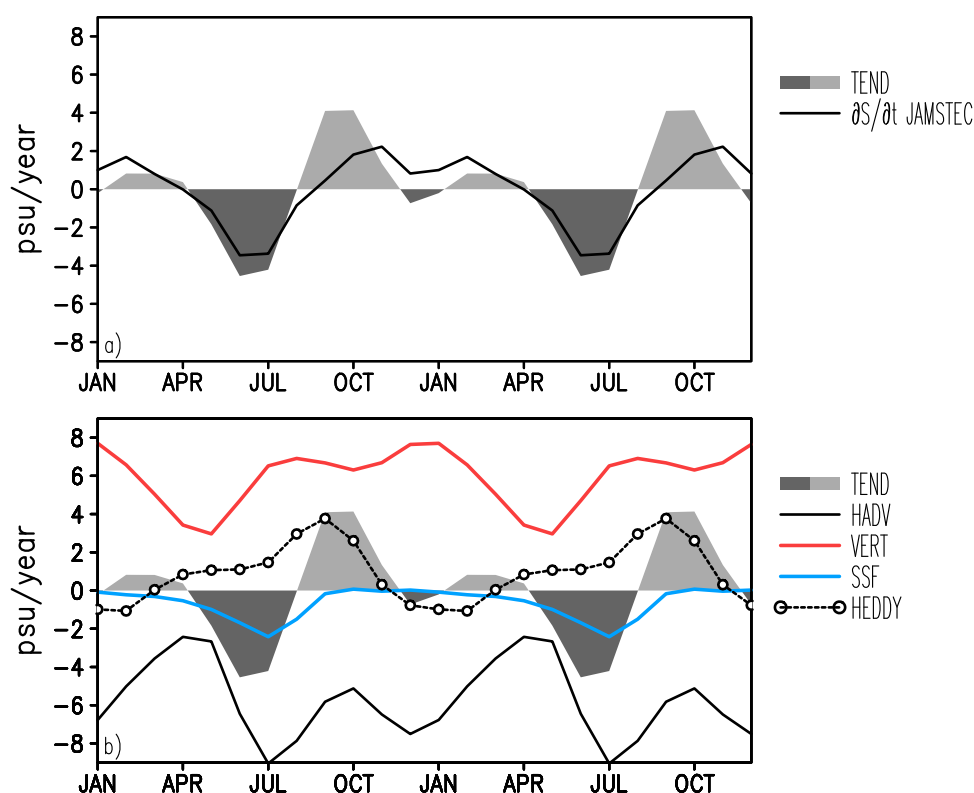
Figure 12. Two years of the seasonal cycle of the simulated mixed layer salt budget terms spatially averaged over the index area shown in Figure 10a: (a) salinity tendency ( TEND = \partial S / \partial t ) and that from JAMSTEC analysis; (b) horizontal salinity advection by mean currents (HADV), vertical processes (vertical advection and turbulent diffusion combined, VERT), surface salt flux normalized by the mixed layer depth (SSF), and horizontal eddy advection (HEDDY).
