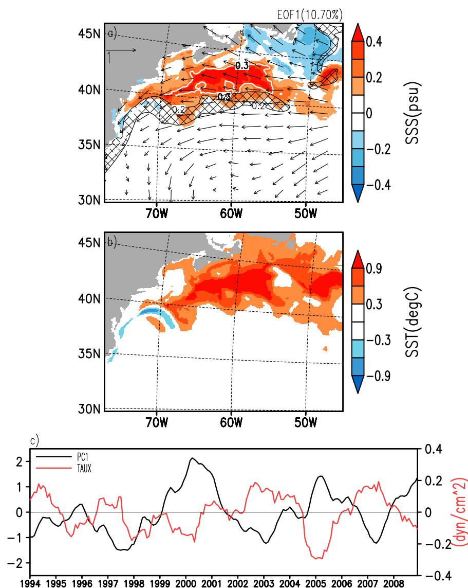
Figure 10. Leading multivariate EOF of monthly anomalous model SSS and SST: (a and b) spatial, (c) temporal components (PC1). In Figure 10a, surface currents >0.2 m/s are cross-hatched, arrows are a temporal correlation of PC1 with 6 month smoothed anomalous wind stress. Anomalous zonal wind stress (TAUX) in Figure 10c is spatially averaged over the index area encompassed by the white contour (0.3 psu) in Figure 10a. It leads PC1 by about 4 months.
